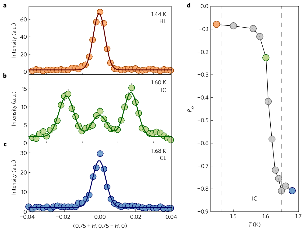
Figure 2 | Multi-step ordering towards the helical ground state. a–c , Neutron diffraction data along the [1\bar{1}0] direction for the (0.75\ 0.75\ 0) reflection measured at 1.44, 1.60, and 1.68 K during cooling. HL, IC, and CL represent the helical, incommensurate and sinusoidally modulated collinear phases, respectively. d , Temperature dependence of the SNP element P_{yy} measured with the (HHL) plane horizontal. Orange, green, and blue points correspond to T=1.44, 1.60 , and 1.68 K, respectively. Error bars represent standard deviations.
