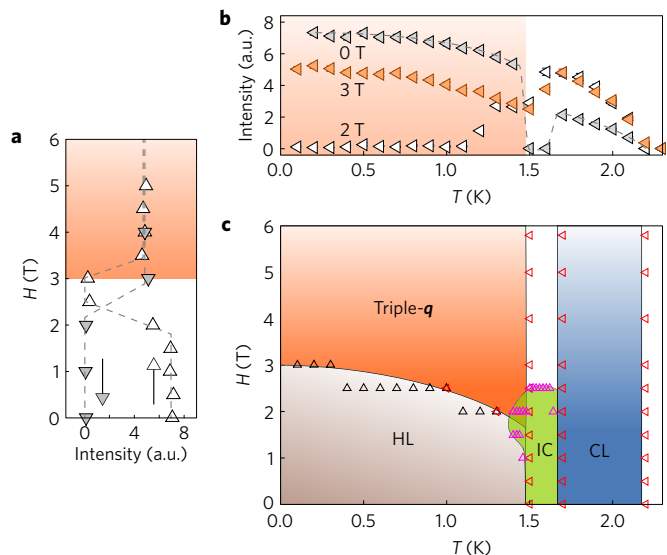
Figure 4 | Phase diagram of \text{MnSc}_2\text{S}_4 under a magnetic field along the [001] direction. a , Field dependence of the intensity of the (0.75 0.75 0) reflection measured at T = 0.1 K. Up-pointing open (down-pointing filled) triangles belong to the measurements with increasing (decreasing) field. b , Temperature dependence of the neutron diffraction intensity of the (0.75 0.75 0) reflection measured under different magnetic fields. c , Phase diagram from neutron diffraction experiments. Up-pointing (left-pointing) triangles mark the transition positions extracted from the measurements with increasing field (decreasing temperature). HL, CL, and IC represent the helical, sinusoidally modulated collinear, and incommensurate phases, respectively. The IC phase disappears under field cooling. Error bars in a,b represent standard deviations and are smaller than the symbol size.
