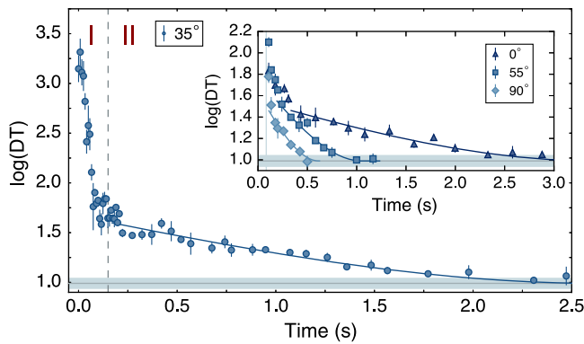
FIG. 3. The full \theta = 35^\circ evolution showing the boundary between regime I and regime II. The solid blue line is fit to the data between the beginning of regime II [ \log(DT) \approx 1.5 ] and the noise floor [ \log(DT) = 1 ]. Vertical bars indicate standard error. The light blue horizontal band is the standard uncertainty of the noise floor. The inset contains regime II decay results for the same angles as in Figs. 2(c)–2(e).
