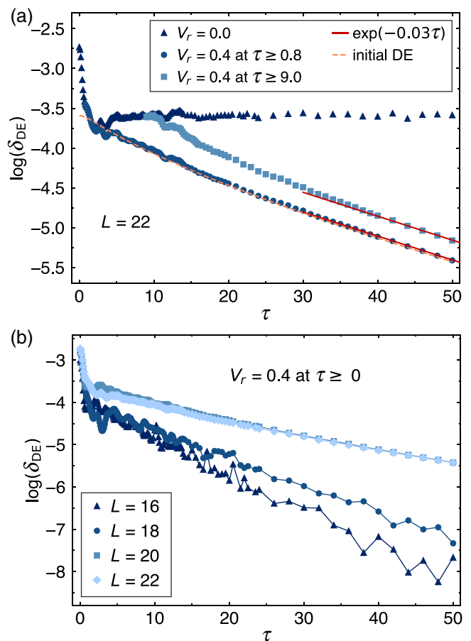
FIG. 18. (a) RMS distance \delta_{\text{DE}}(\tau) [defined in Eq. (9)] versus \tau for two-step quenches in which V = 1.6 , V_r = 0.4 , and L = 22 . The distance is computed, in all cases, from the DE result for the single quench. Results are shown when the second quench is carried out at \tau = 0.8 and 9.0 following the first quench, and at \tau = 0 when starting with the DE of the integrable system after the first quench (labeled as “initial DE”). The solid lines at long times depict exponential behavior indicating the same relaxation rate in all cases. (b) Distance to equilibration in single quenches for different systems sizes L . These results show the finite-size effect on the relaxation rates.
