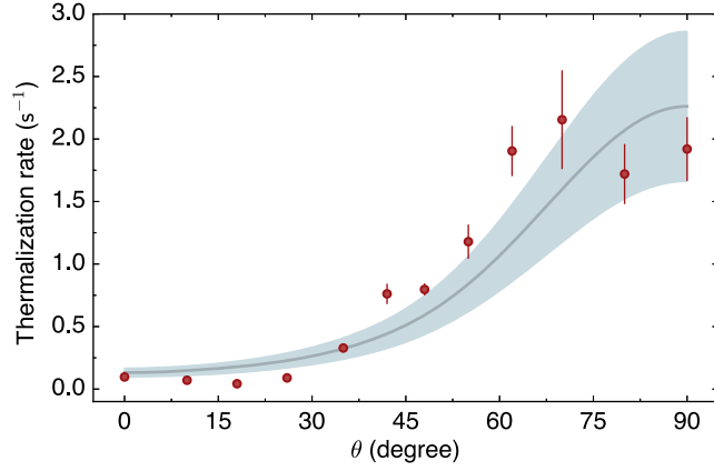
FIG. 4. Thermalization rate data in red versus \theta . See Eq. (1) for the definition of the thermalization rate 1/\tau_{\text{th}} . The gray curve is the scaling estimate \gamma^2(\theta)U_{\text{total}}^2(\theta)/(E_c) with no free parameters or offset. Vertical bars and the light blue band indicate standard error; atom number noise and a_{3\text{D}} uncertainty dominate the latter. Evidently, the thermalization rate in the dipolar quantum Newton's cradle is well described by terms dependent on both the long-range and short-range parts of the DDI, the former through total (intertube plus intratube) U_{\text{total}}^2(\theta) and the latter through the intratube DDI dependence of a_{\text{ID}}^{\text{intra}}(\theta) in \gamma^2(\theta) .
