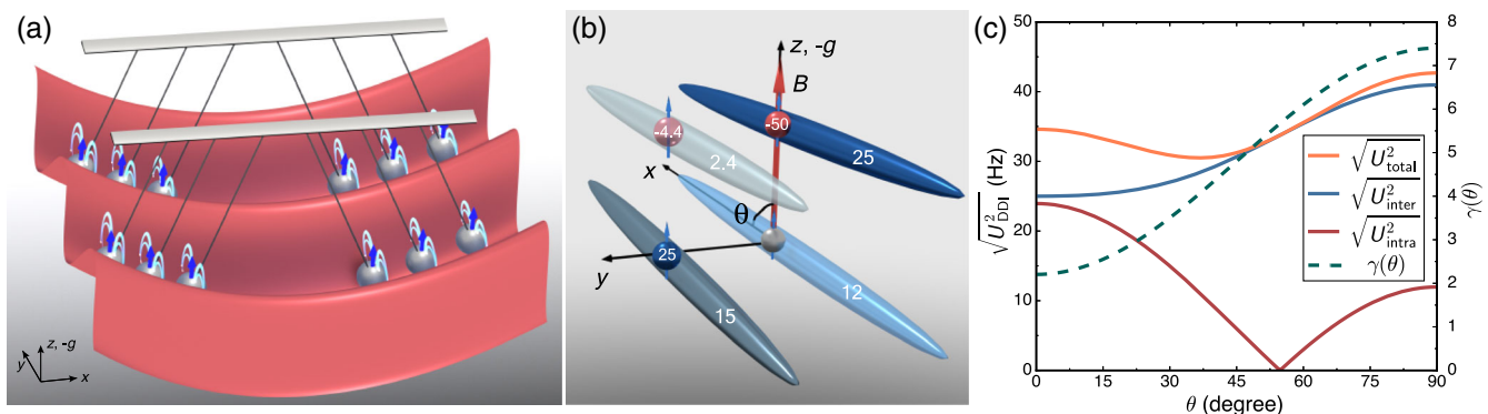
FIG. 1. Dipolar Newton’s cradle setup. (a) Two of the 1D tubes of atoms in a dipolar quantum Newton’s cradle. Application of an optical phase grating (not shown) kicks atoms along the tubes, and the weak harmonic confinement induces periodic collisions. The highly magnetic dysprosium atoms (silver spheres) are trapped in a 2D optical lattice (red) defining the tubes. (b) DDI strength between the central atom and atoms in neighboring tubes in one quadrant of the square lattice when \theta = 90^\circ , where \theta is the angle between the B-field in the xz -plane and the axis of the 1D tubes along \hat{x} . The patterns of strengths in the other three quadrants are the same by symmetry. The DDI strength is tunable via changing \theta . Numbers labeled on the atoms and the tubes are the pairwise DDI strength and integrated DDI along the tubes, respectively, in Hz. Blue indicates large positive strength, and red large negative strength. (c) Dependence of integrability-breaking dipolar interaction strength and \gamma on \theta . Solid curves: Integrability-breaking contributions of the DDI energy U_{\text{DDI}} (added in quadrature and defined in Appendices A–C) versus \theta . Shown are the total, total intertube, and total integrability-breaking intratube DDI energies. While the intratube DDI is maximally repulsive (attractive) for \theta = 90^\circ ( 0^\circ ), it vanishes among intratube atoms for \theta = 55^\circ . Integrability-breaking DDI contributions come not just from the intratube 1D DDI along \hat{x} , but also from the 3D DDI between atoms in all neighboring tubes along \hat{y} and \hat{z} . This dilutes the tunability of the DDI, reducing the contrast to a factor of approximately 1.5 between \theta = 0^\circ and 90^\circ . Dashed curve: Lieb-Liniger parameter \gamma(\theta) ; see Appendix D for calculation.
