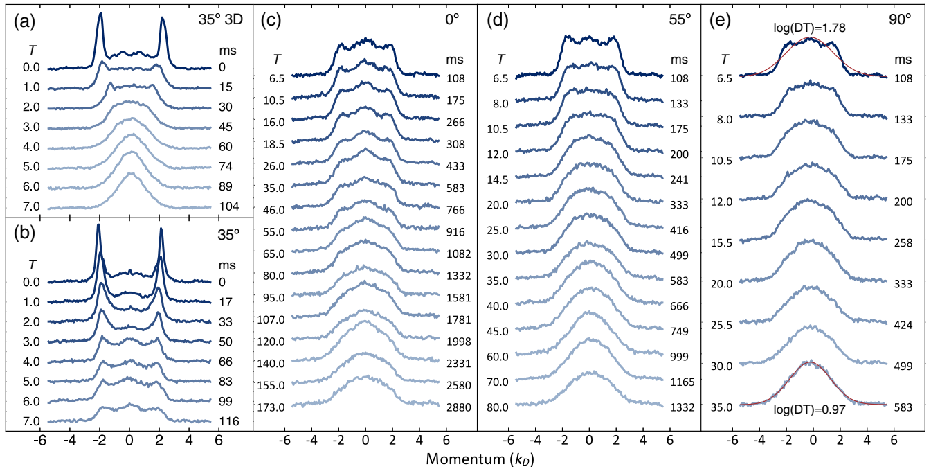
FIG. 2. Evolution of postkick momentum distributions at multiples of T . (a) 3D gas at \theta = 35^\circ . (b) Regime I, fast dephasing of the 1D gas at \theta = 35^\circ . While the momentum distribution of the 3D gas thermalizes after about 5T , the 1D gases exhibit nonthermal (i.e., non-Gaussian) distributions far longer. The remaining panels show 1D gases in regime II for \theta 's of (c) 0^\circ ; (d) 55^\circ ; and (e) 90^\circ . We diffract and evolve with \theta = 35^\circ until rotation at 5T to the target \theta . As can be seen in panels (c)–(e), this procedure produces nearly identical momentum distributions after field rotation regardless of \theta . The color scale is proportional to the distance to thermalization. The best-fit Gaussian curve and the corresponding \log(DT) value are shown for the 90^\circ data at the earliest and latest times.
