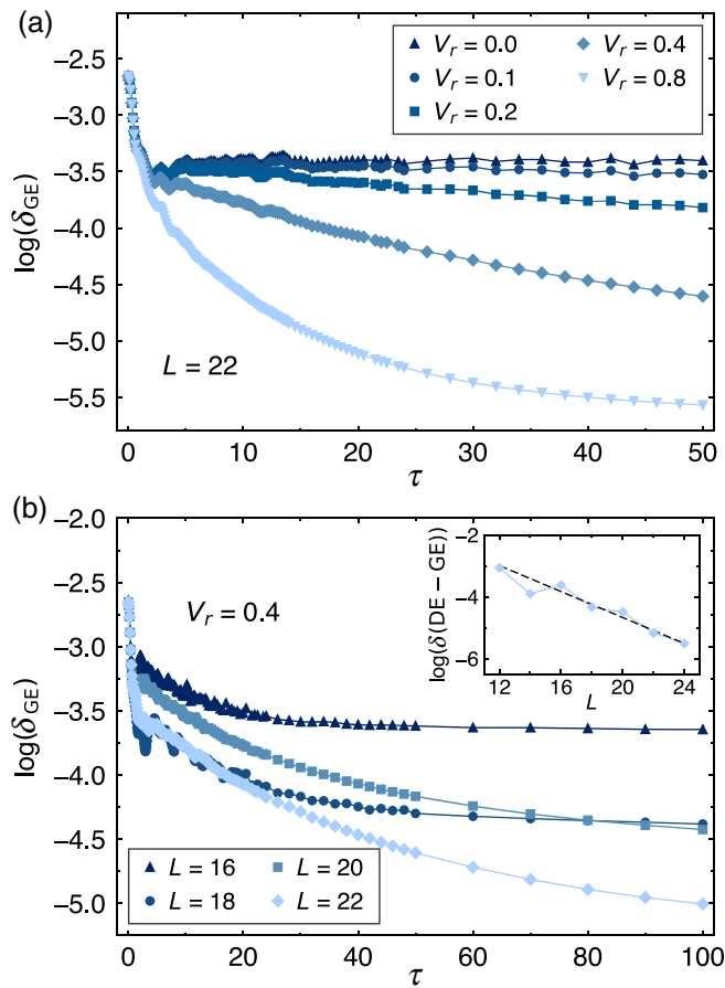
FIG. 17. (a) RMS distance \delta_{\text{GE}}(\tau) [see Eq. (L4)] versus \tau for quenches in which V = 1.6 and the integrability breaking V_r takes different values. The results shown are for a system with L = 22 sites. (b) RMS distance \delta_{\text{GE}}(\tau) versus \tau for quenches in which V = 1.6 , V_r = 0.4 , and for different lattice sizes ( L = 16, 18, 20 , and 22 ). Inset in (b): Distance between the diagonal and the grand canonical ensembles \delta(\text{DE}-\text{GE}) [see Eq. (L5)] versus L for V = 1.6 and V_r = 0.4 (as in the main panel). The black dashed line depicts exponential behavior.
