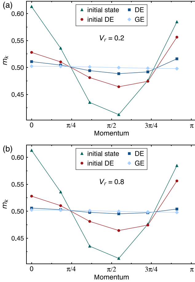
FIG. 16. Examples of momentum distributions ( m_k ) obtained in the exact diagonalization calculations of the two-rung hard-core boson model with L = 22 . We show the momentum distributions for an initial state (labeled as “initial state”), the diagonal ensemble after the quench to the integrable part of \hat{H}_F (labeled as “initial DE”), the diagonal ensemble after the quench to \hat{H}_F (labeled as “DE”), and the grand canonical ensemble prediction for the thermal momentum distribution after the quench (labeled as “GE”). For the quenches, we set V = 1.6 , with (a) V_r = 0.2 and (b) V_r = 0.8 . The momentum distribution of the initial state and of the diagonal ensemble after the quench to the integrable part of \hat{H}_F are the same in (a) and (b); only the diagonal and grand canonical ensemble predictions change due to the change of V_r .
