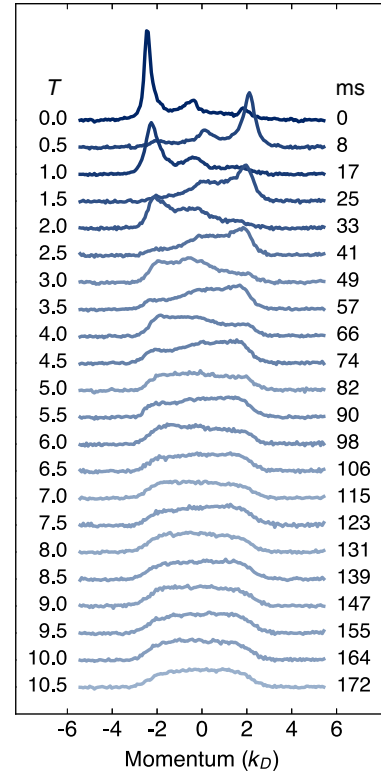
FIG. 14. Time evolution of an initially single-sided momentum distribution, whose dephasing timescale accounts for the technical dephasing mechanisms while minimizing those from high-energy collisions.
