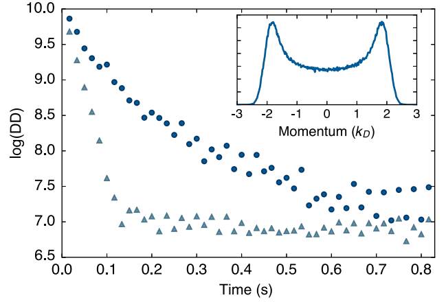
FIG. 12. Time evolution of distance to dephasing (DD) predicted by the collisionless classical dynamics simulation for two cases: the first for when only process (ii) is present (circle), and second when both (i) and (ii) are present (triangle). The inset shows the dephased momentum distribution.
