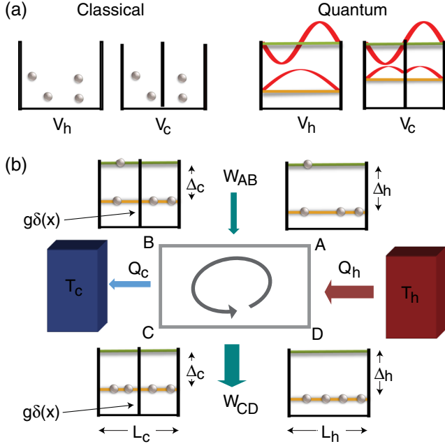
FIG. 1. (a) The adiabatic introduction of an infinite \delta function barrier does not change the energy of a classical ideal gas (left), precluding classical work extraction, but shifts the energy of the quantum ground state (right) due to the nonzero amplitude of its wave function at the barrier position, enabling quantum work extraction. (b) A quantum Otto cycle heat engine using the infinite well potential and the \delta barrier. The cycle is composed of two adiabatic strokes (connecting states A and B, and C and D) where the potential is adiabatically deformed and the ion does not interact with any thermal bath, and two “isochoric” or “isoparametric” strokes [31] (connecting states B and C, and D and A) where the potential is kept constant while the ion equilibrates with the cold and the hot bath, respectively see the SM [35] Sec. VII. Work exchange results from the energy shift of the ground state, while the excited state remains unshifted (for L_c = L_h ): work extraction W_{CD} takes place after thermalization with the cold bath and therefore at high ground-state population, whereas work injection W_{AB} takes place after thermalization with the hot bath and therefore at lower ground-state population. The difference between the ground-state populations results in net work extraction |W_{CD}| > |W_{AB}| at constant volume [36].
