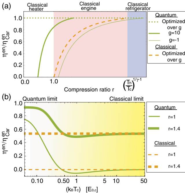
FIG. 2. (a) Efficiency normalized to Carnot efficiency for a classical (see SM [35] Sec. III) and quantum (see SM [35] Sec. I) Otto engine with a barrier of the form g\delta(x) [see Fig. 1(b)]. The plane is divided into three areas depending on the classical operation mode [see Eq. (1) and the discussion below it]. The temperature ratio is (T_h/T_c) = 12 , \gamma = 3 , g is given in units of the critical value g_{\text{cri}} = (2\hbar^2/mL_c) , and units are assumed such that (2\hbar^2/mL_h) = 1 . (b) Classical (dashed) and quantum (continuous) normalized efficiency as function of T_c , for r = 1.4 (thick) and r = 1 (thin), and fixed ratio (T_h/T_c) for an ideal gas. The temperature dependence is a signature of the quantum machine. The number of populated levels depends on the temperature.
