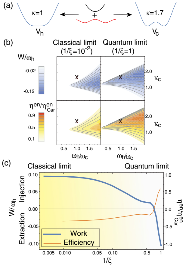
FIG. 3. (a) The proposed experimental potential [see Eq. (4)]. (b) The calculated work (top) and normalized efficiency (bottom) for the classical (left) and quantum limit (right). Here \kappa_h = 1 and \omega_h = 1 MHz have been chosen. The white areas correspond to the heater. The X indicates the parameters used for Fig. 3(c), \kappa_c = 1.7 and \omega_c = \omega_h , where the classical heater operates as a heat engine in the quantum limit. (c) The calculated work and efficiency. The classical limit is obtained at (1/\xi) \rightarrow 0 , where the work becomes constant and positive (work injection). In contrast, at the quantum limit, (1/\xi) = 1 , work is extracted. Cycle parameters: T_h/T_c = 41.6 , \bar{n}_c = 0.033 .
