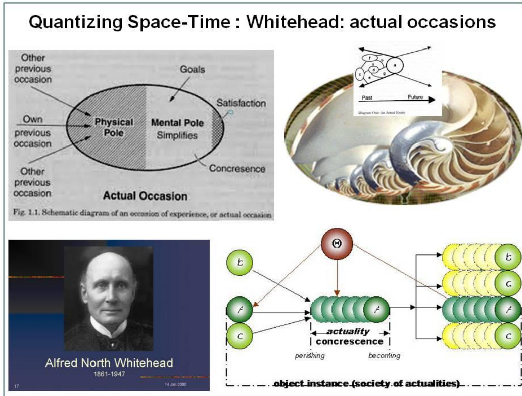
Fig. 14 : Quantizing space time of Whitehead by postulating units of experience and actual occasions that have a mental and physical pole and carry elements of goals, satisfaction and beauty. They are build up from previous occasions from societies of occasions( right insets).
