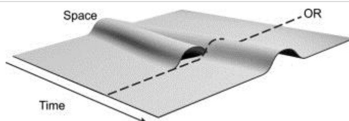
Fig. 19: As superposition curvature E reaches threshold, OR occurs and one particle location/curvature is selected, and becomes classical. The other ceases to exist.
