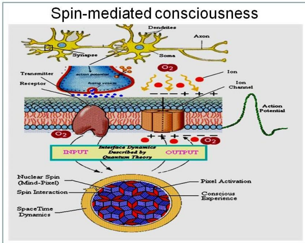
Fig. 34: The plasma membrane structure and membrane potential of neurons exhibiting channel proteins that enable electric activity through trans-membrane flux of Na- an K-ions, that may be influenced by quantum spin information of the constituting elementary particles of channel proteins.
