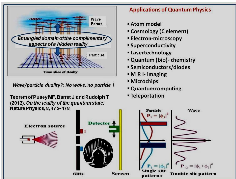
Fig. 5: Wave/ particle duality in Quantum physics should be rather seen as a state in which a particle and wave forms are complementary features in an hidden reality (up left), and Pusey et al showed that the wave form is a physical reality (middle left). Principles of Quantum physics are presently used in a large variety of technologies (up right). The conscious observer or a detector that observes the double slit system and provides interpretable data collapses the wave function to a single slit pattern.
