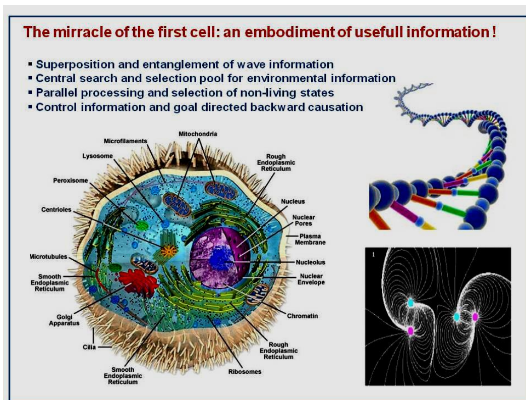
Fig. 52: Potential quantum mechanisms in the evolution to first life
